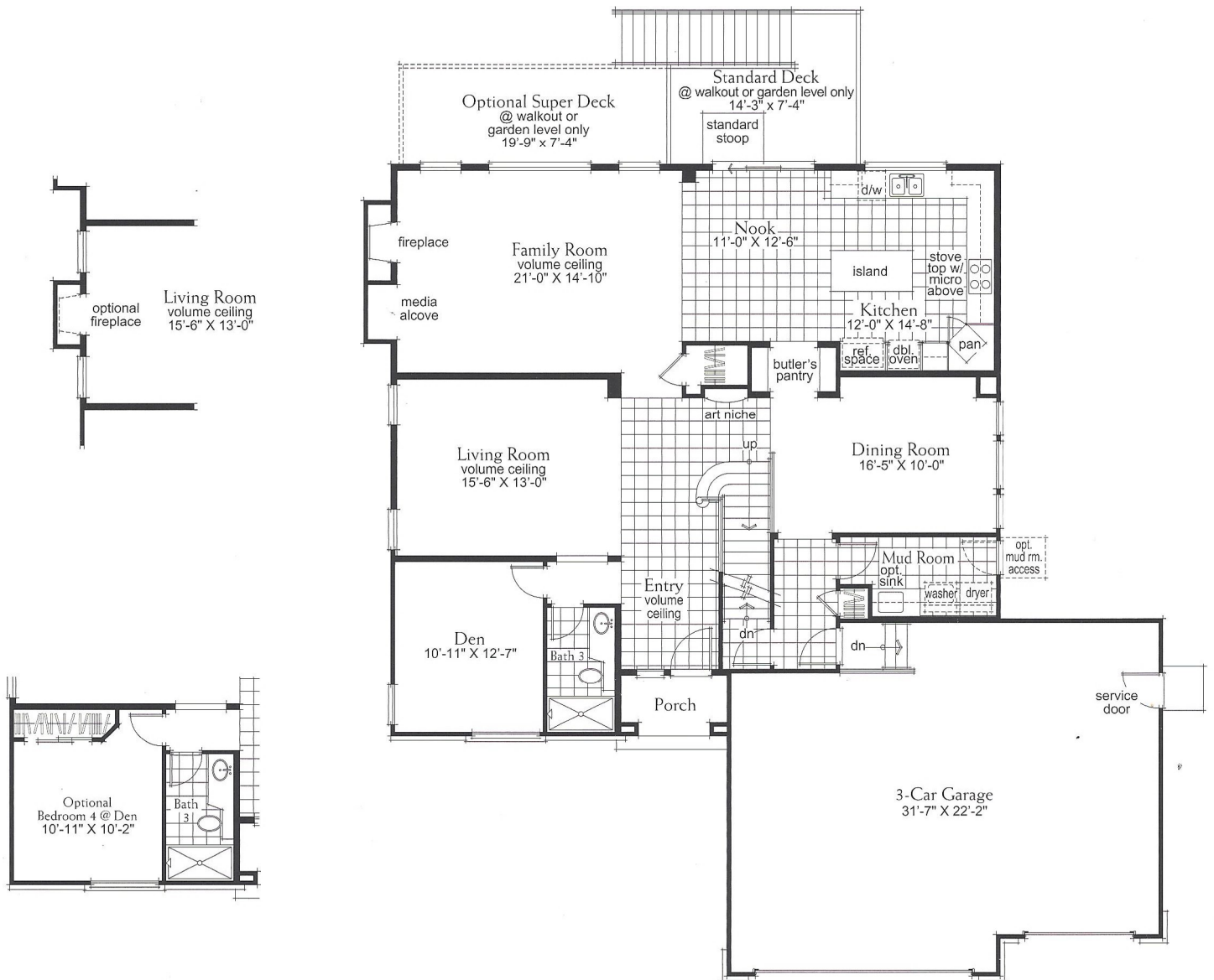
First Floor
